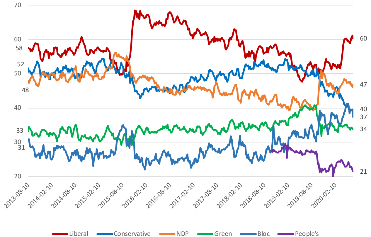
Canada Weekly Index Tracking Scores (Ending June 26, 2020, n=1,000)
